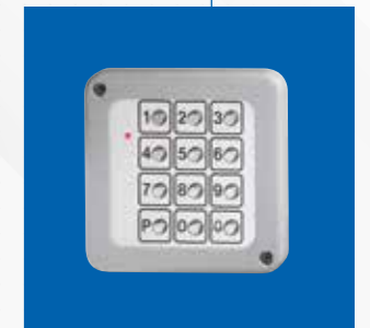
Coded key pad signal 213 3 signals, metal key pad, 230 V connection
